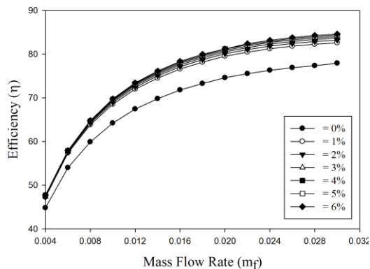
Fig. 8 Average thermal efficiency for (WBFPS) and (NBFPS) as a function of working fluid mass flow rates during a typical
