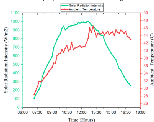
Fig. 6 Solar radiation and Ambient temperature Vs Time
