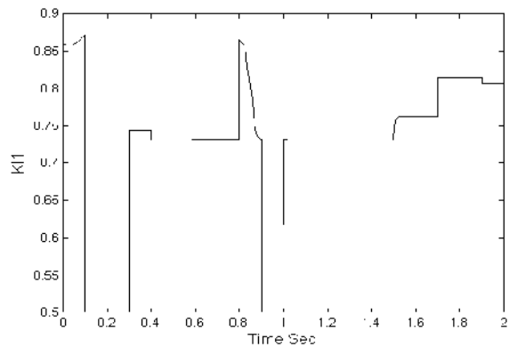
Fig.12: gain ( K_{I1} ) varies online with the output of the system under control.
