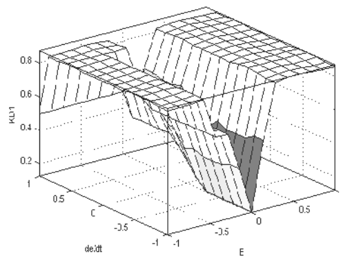
Fig.16: Rule surface viewer of K_{D1} .
