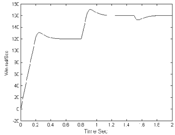
Fig.9.c: Motor speed ( \omega_m ) using conventional PID controller.
