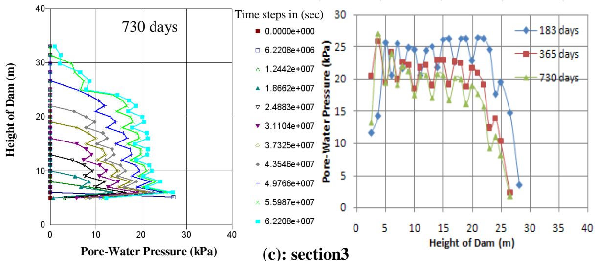
Figure (9): Pore pressure development during different construction stages
