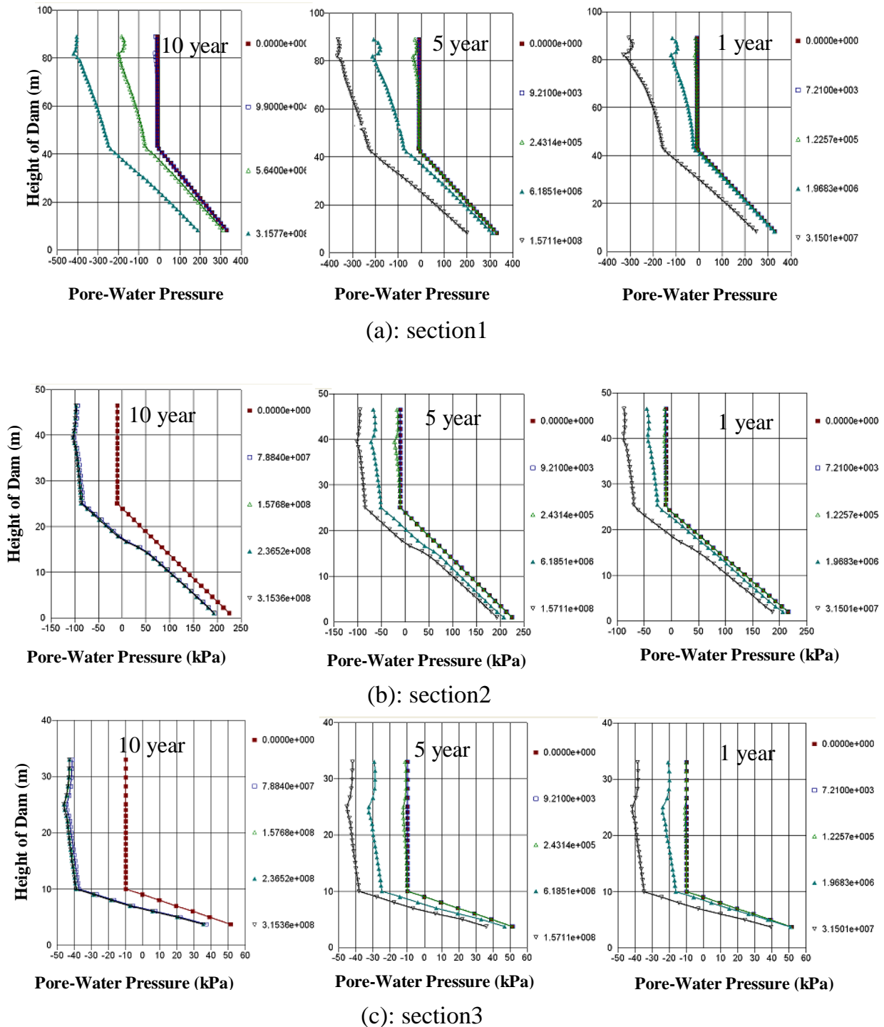
Figure (12): Pore pressure development at minimum water level
