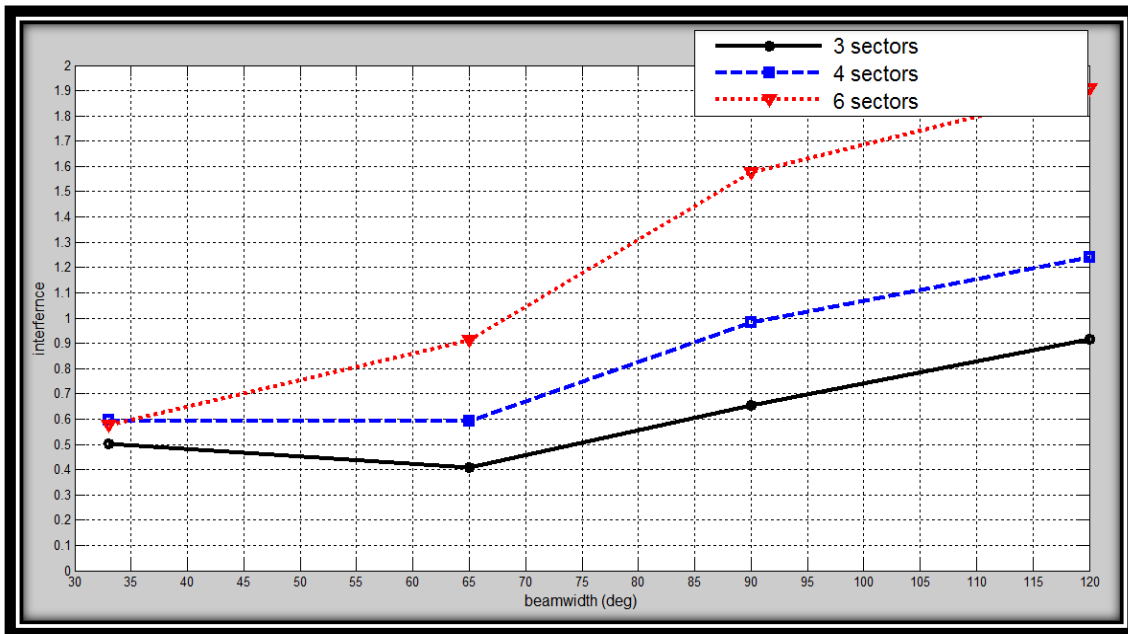
Figure (14) Impact of the antenna beamwidth on interference
