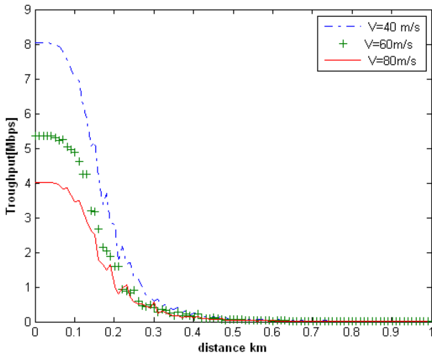
b- Effect of speed in WiFi AP
