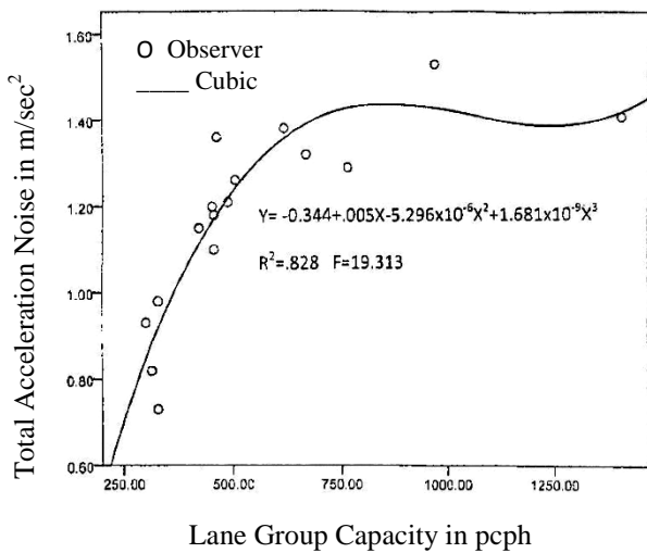
Figure (5): Effect of Lane Group Capacity in pcp on the Total Acceleration Noise in m/sec 2 at Signalized Intersections
