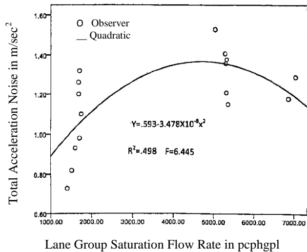
Figure (6): Effect of Lane Group Saturation Flow Rate in pchgpl on the Total Acceleration Noise in m/sec 2 at Signalized Intersections
