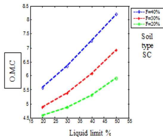
Figure (10) Effect of LL and fine material on O.M.C (soil type SC)
